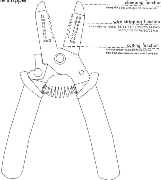
Wire stripper
